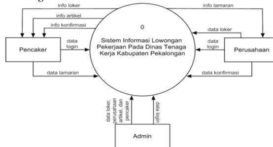
Gambar 1. Diagram Context
